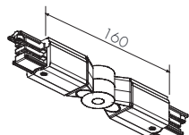
[ Adjustable corner connector ] XTS 24
